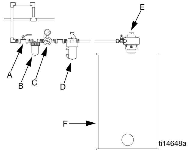
FIG. 2: Installation type
